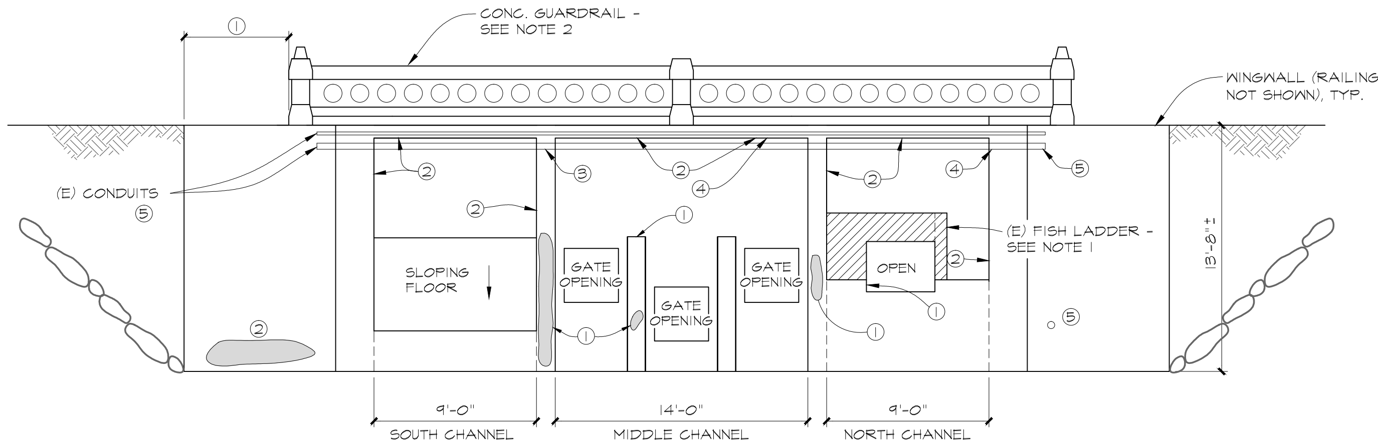
2 ELEVATION FACING UPSTREAM SCALE: 3/16"=1'-0"
