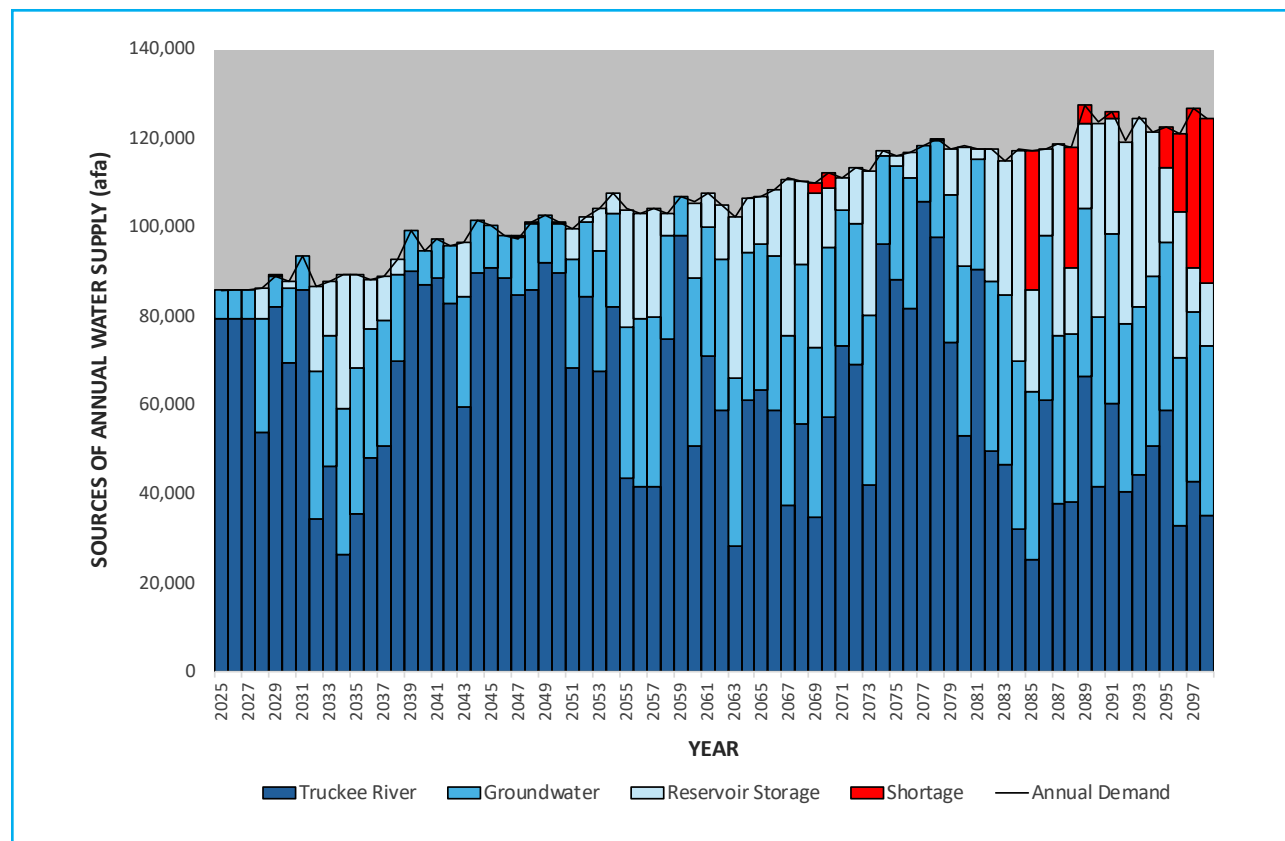
FIGURE 3-9: TMWA PROJECTED ANNUAL SOURCES OF SUPPLY THROUGH 2098 UNDER RCP 8.5 WITHOUT ASR
