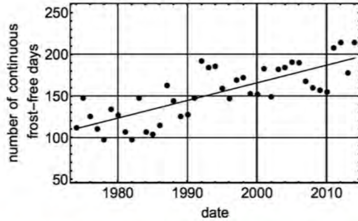
FIGURE 5: Trend in the growing season (see text for definition) in Reno, Nevada over the past 41 years (KRNO data).
