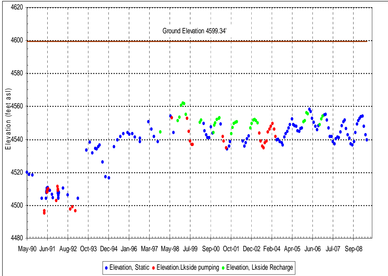
Figure 3. Bartley Ranch, Historical Water Level Elevations
