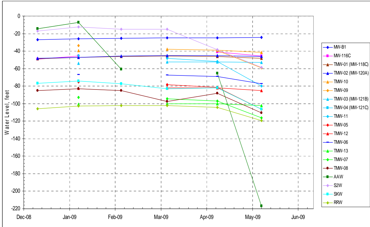
Figure 5A. West Lemmon Valley Wells, 1 st Half 2009 Water Levels
