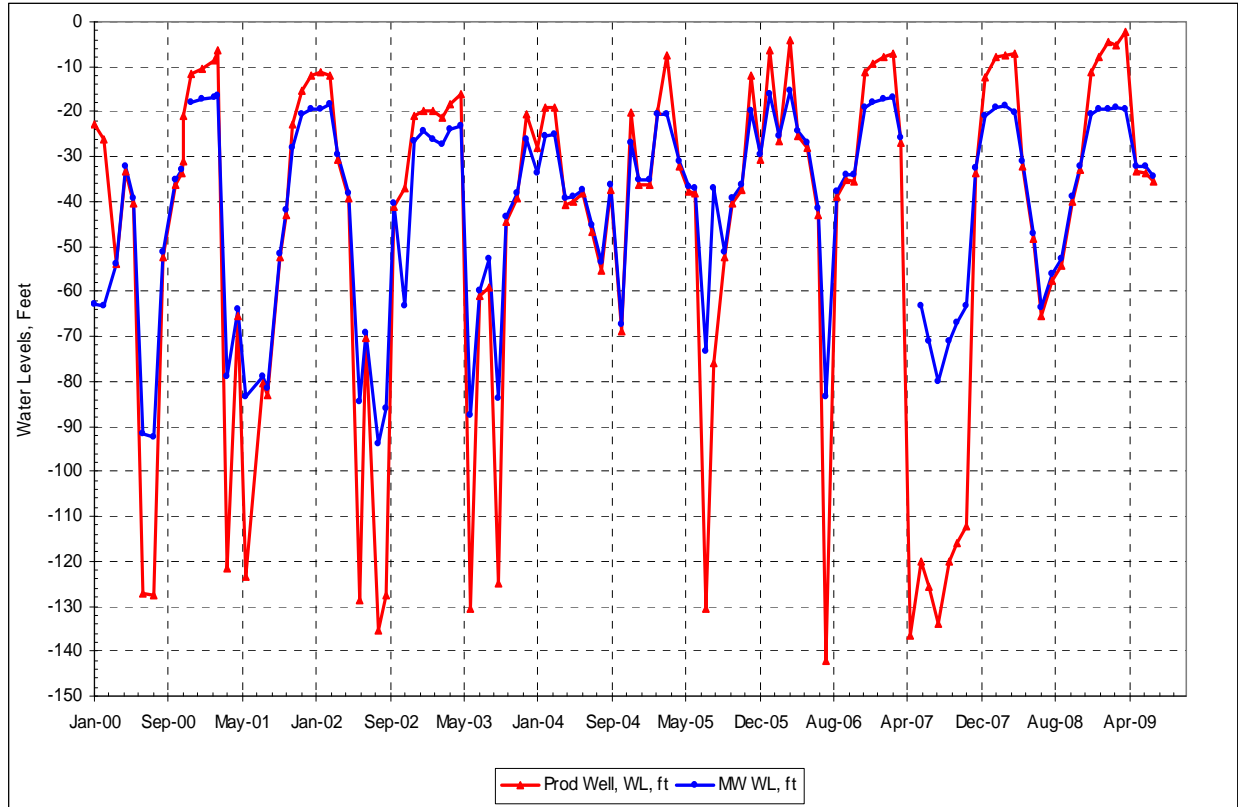
Figure 15. Galletti Way Production and Monitoring Wells, Historical Water Levels
