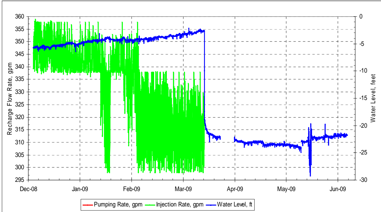
Figure 8A. Reno High Well - Mean Hourly Water Levels and Flow Rates, First Half 2009
