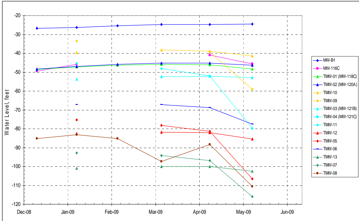
Figure 6. West Lemmon Valley Monitoring Wells, 1 st Half 2009 Water Levels
