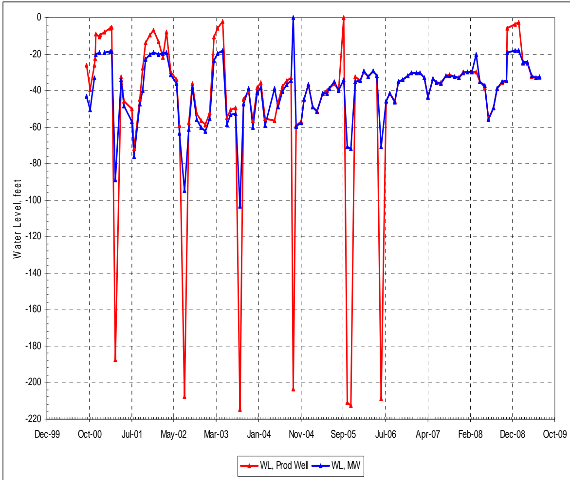
Figure 18. Glen Hare Injection and Monitoring Wells - Water Levels
