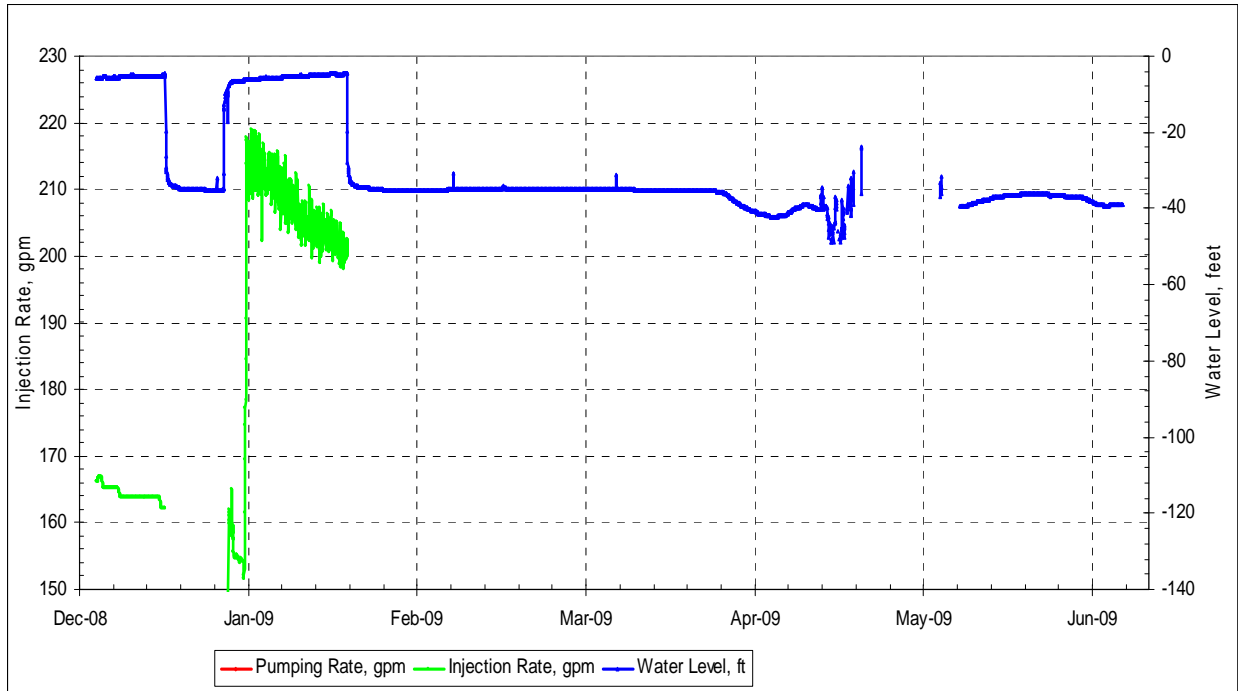
Figure 19A. Holcomb Lane Well – Water Levels and Injection Rates, 1 st Half 2009
