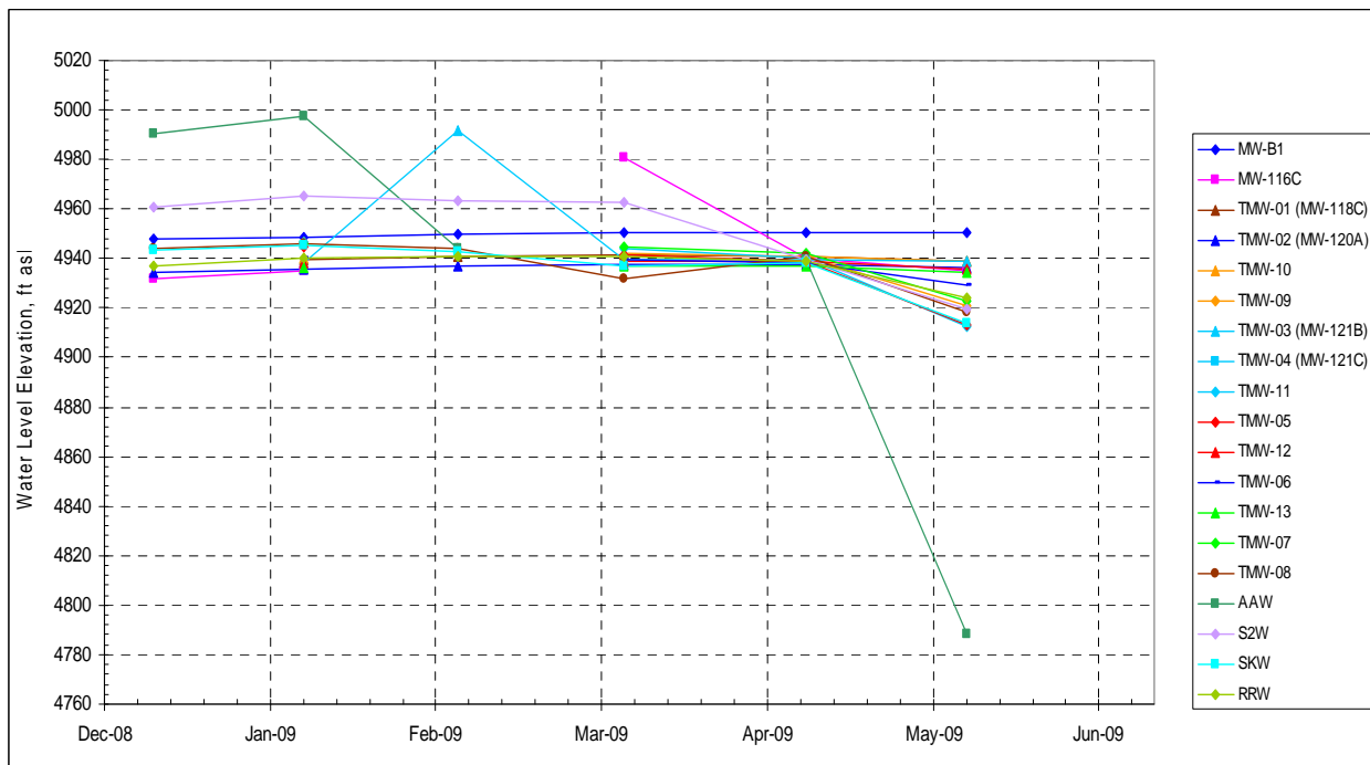
Figure 5B. West Lemmon Valley Wells, 1 st Half 2009 Water Level Elevations
