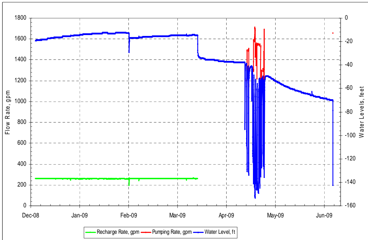
Figure 3. Silver Lake Well, 1 st Half 2009 Flow Rates and Water Levels
