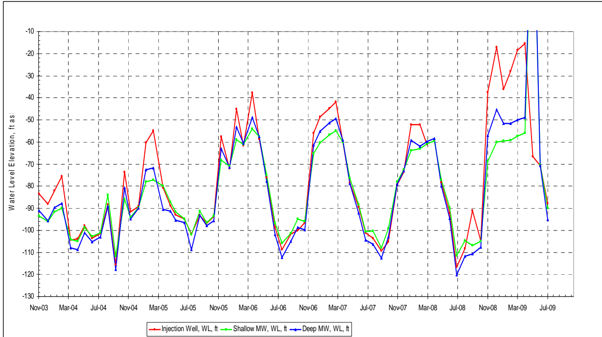
Figure 11. 4th Street Injection and Monitoring Wells, Water Levels
